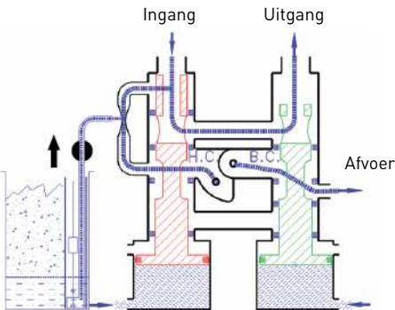
Schema pekelaanzuiging
